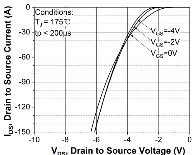
Figure 10. Body diode characteristic at T_J = 175^\circ C
