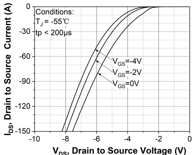
Figure 8. Body diode characteristic at T_J = -55^\circ C
