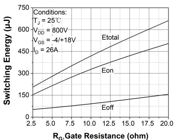
Figure 25. Clamped inductive switching energy vs. R_G (ext)
