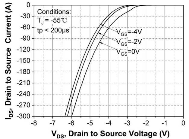
Figure 8. Body diode characteristic at T_J = -55\text{ }^{\circ}\text{C}
