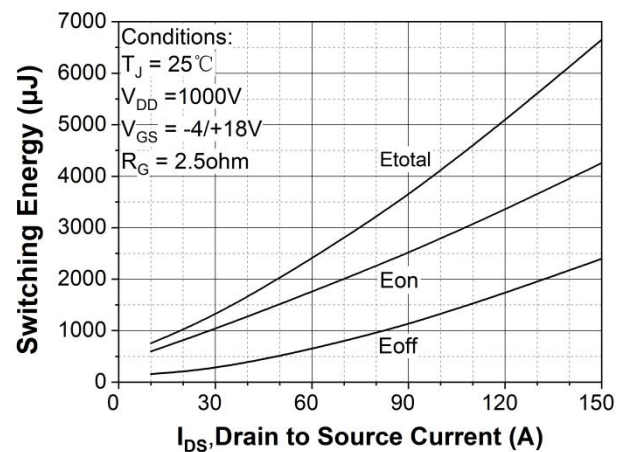
Figure 24. Clamped Inductive switching energy vs. drain current ( V_{DD} = 1000\text{V} )
