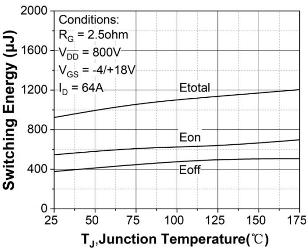
Figure 26. Clamped inductive switching energy vs. temperature
