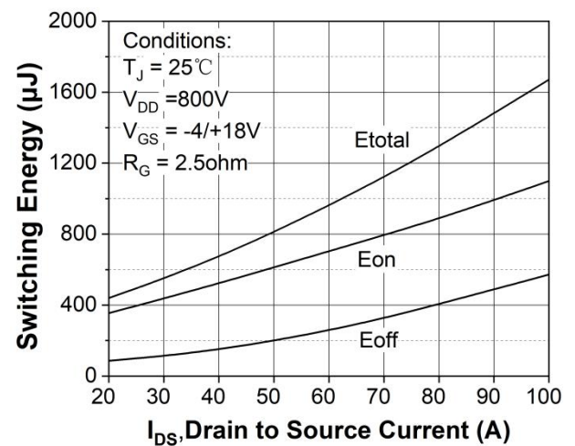
Figure 24. Clamped inductive switching energy vs. drain current ( V_{DD} = 800\text{V} )
