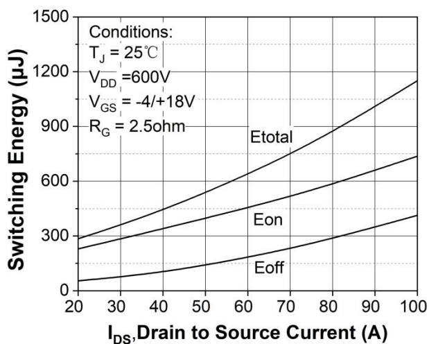
Figure 23. Clamped Inductive switching energy vs. drain current ( V_{DD} = 600\text{V} )
