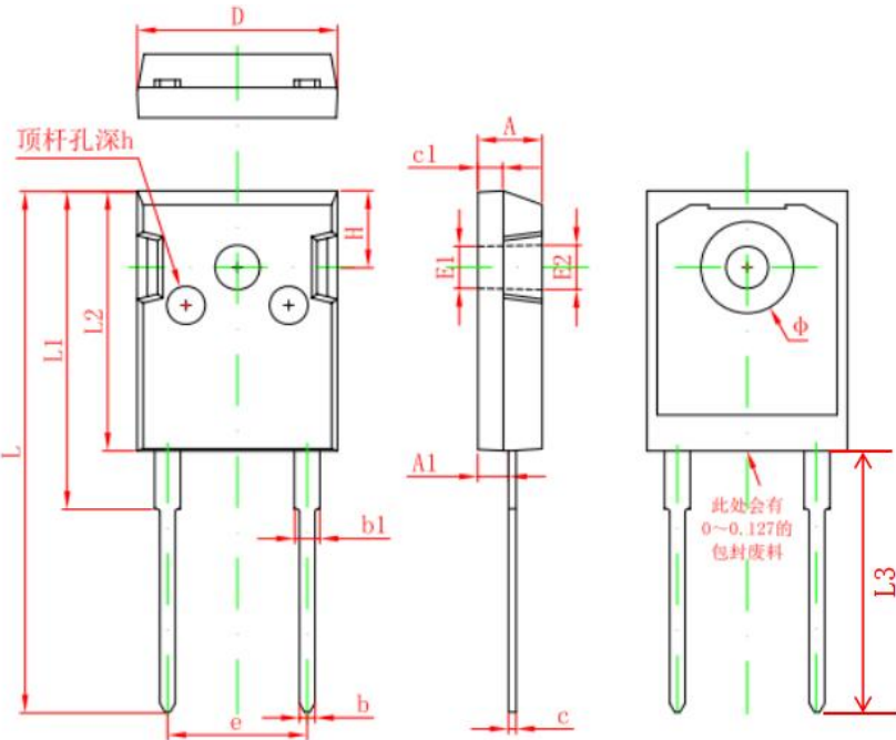
TO-247-2L-A
