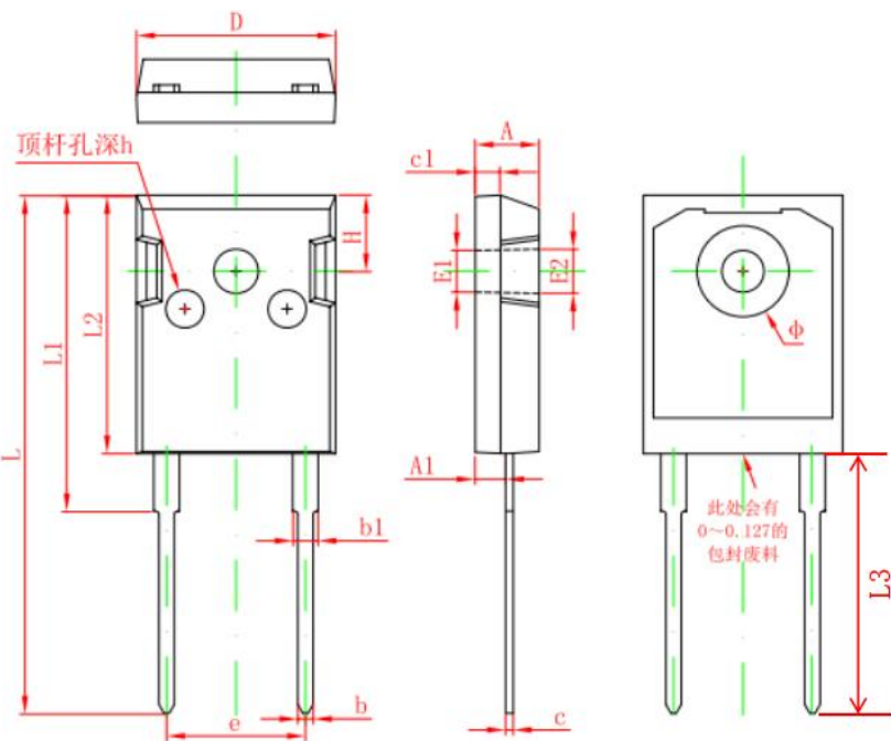
TO-247-2L-A
