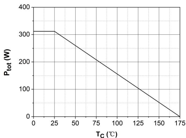
Figure 6. Power Derating
