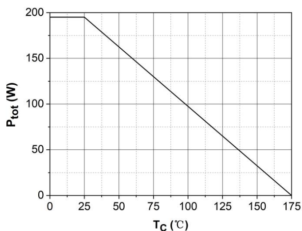
Figure 6. Power Derating
