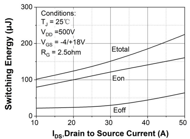
Figure 24. Clamped inductive switching energy vs. drain current ( V_{DD} = 500\text{V} )
