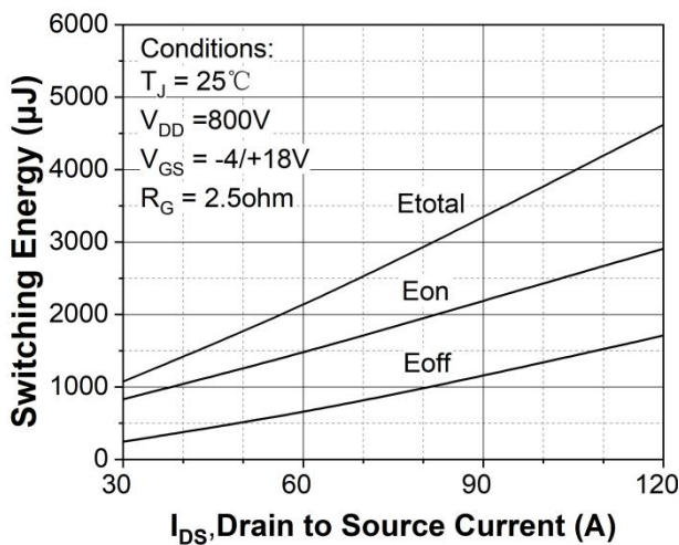
Figure 23. Clamped inductive switching energy vs. drain current ( V_{DD} = 800\text{V} )
