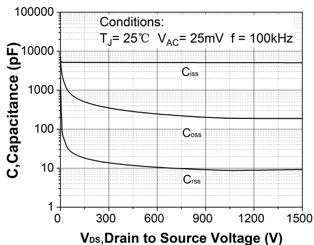
Figure 18. Capacitances vs. drain-source voltage (0 - 1500V)
