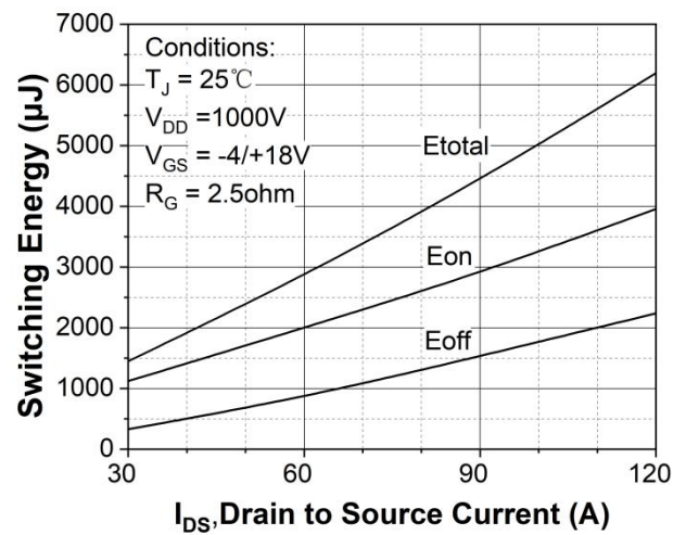
Figure 24. Clamped inductive switching energy vs. drain current ( V_{DD} = 1000\text{V} )
